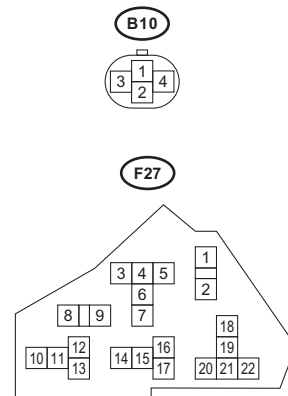
RELAY HOLDER
