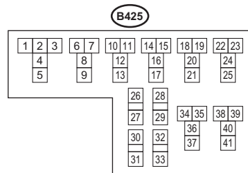
RELAY BLOCK
