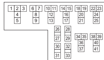
RELAY BLOCK
