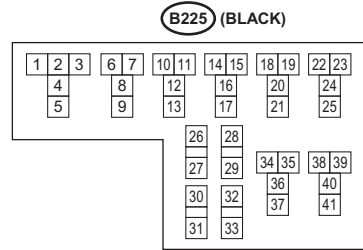
RELAY BLOCK
