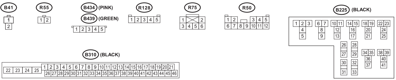
RELAY BLOCK
