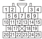
REAR DOUBLE LOCK ACTUATOR LH
