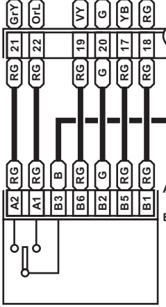
FRONT DOUBLE LOCK ACTUATOR RH & DOOR KEY SWITCH
